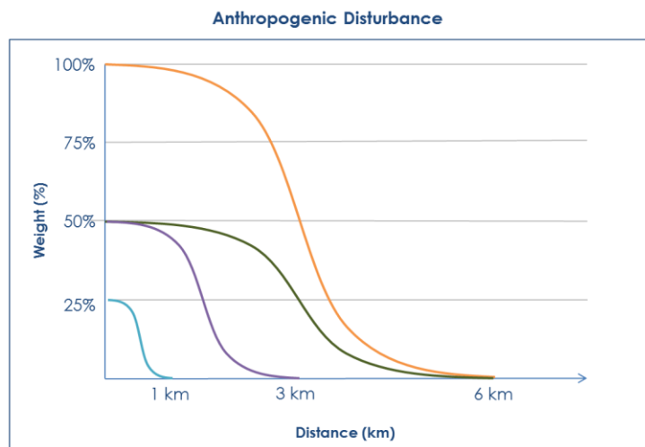
Figure 6: Example distance-decay curves with the y-intercept the weight and the x-intercept the distance associated with the anthropogenic disturbances.
