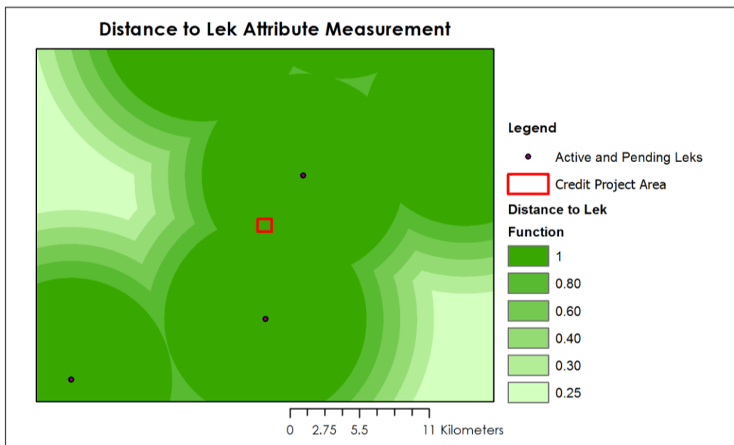
Figure 11. Effect of Distance to lek attribute on breeding habitat function for an example credit project
