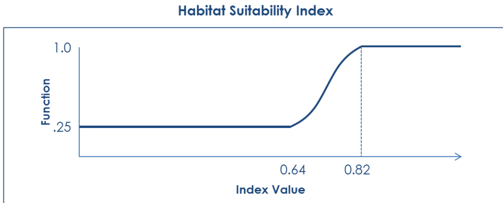
Figure 8. Scoring curve for the HSI attribute as a local-scale modifier of habitat function
