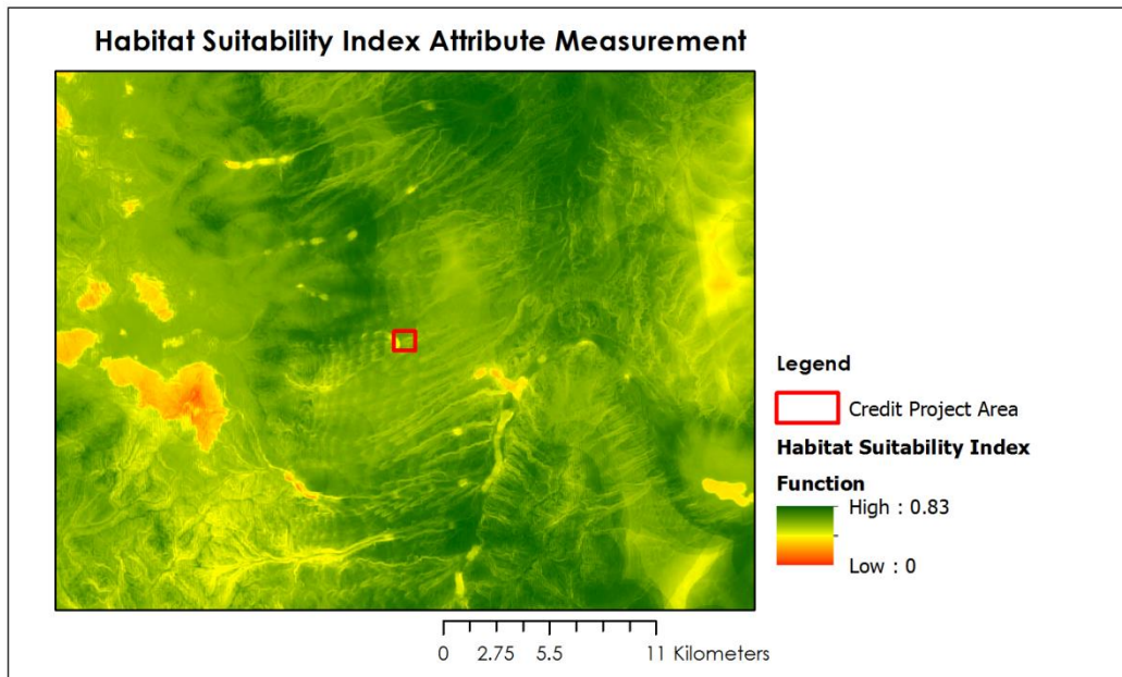
Figure 9. Habitat suitability related to the HSI in the area surrounding an example credit project site
