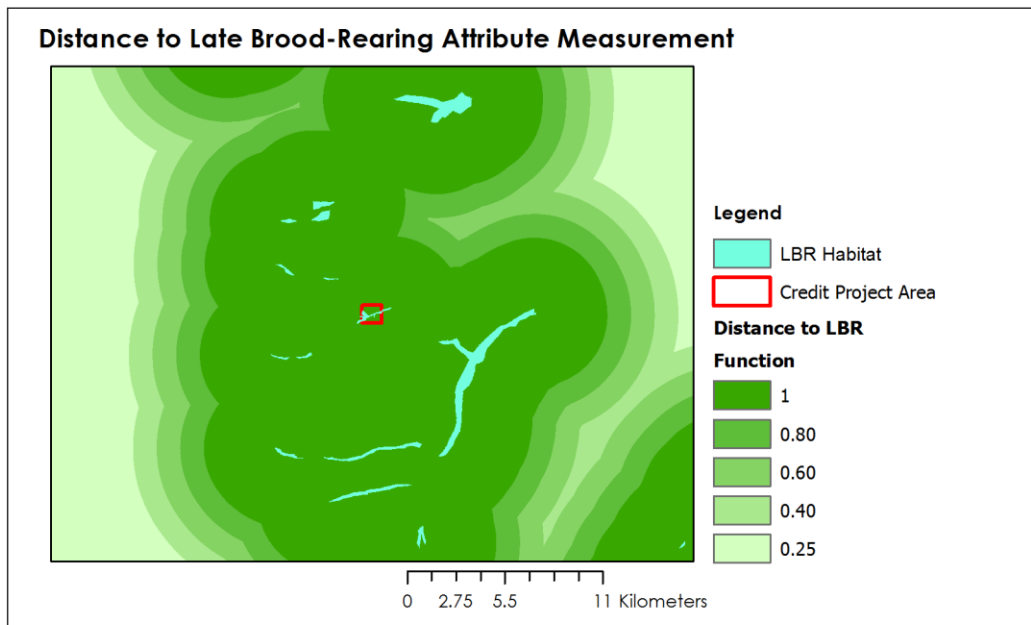
Figure 13. Effect of distance to late brood-rearing attribute on breeding habitat function for an example credit project
