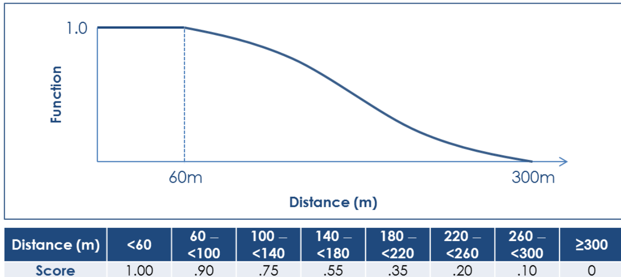
Figure 18. Scoring curve and table for scoring late brood-rearing habitat based on distance to sagebrush cover
