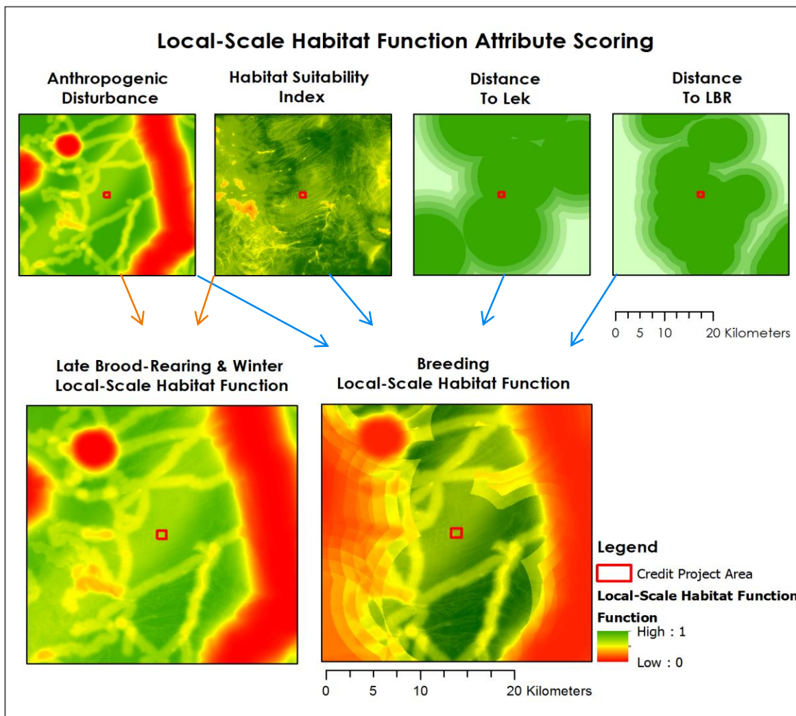
Figure 14. Local-scale attributes are measured in a GIS and combined to calculate local-scale habitat function for each seasonal habitat type.
