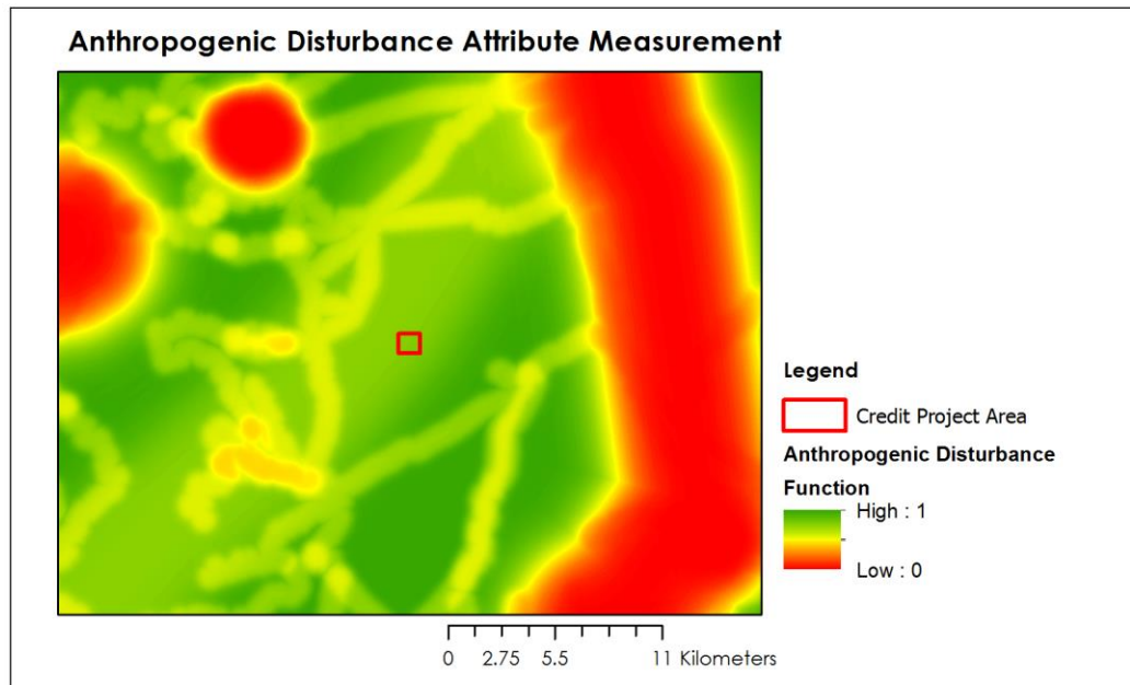
Figure 7: Indirect effects of anthropogenic disturbance on sage-grouse habitat as visualized in a continuous surface raster in the area surrounding an example credit project site
